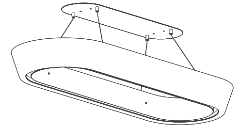
Suspended light with 4 wire cables Suspended depth: 500 – 1500 mm
